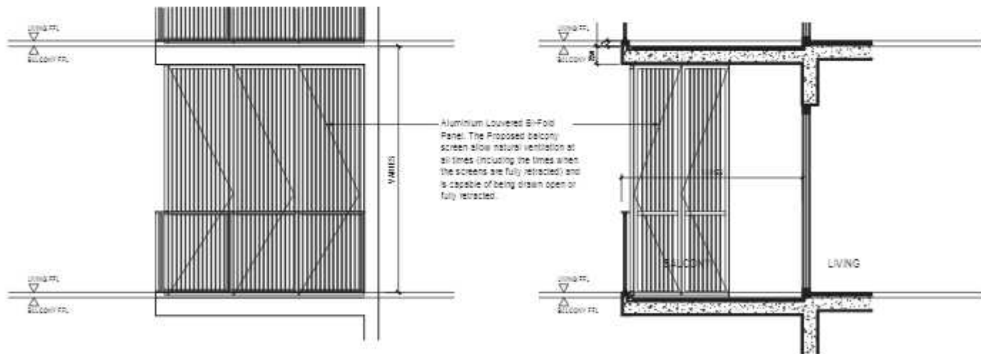
TYPICAL RETRACTABLE BALCONY SCREEN - ELEVATION
